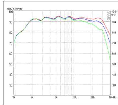
SPL HORIZONTAL 0° - 15° - 30°
