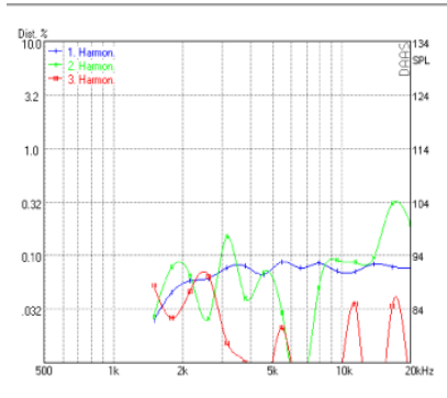
Harmonic Distortion 2.83 V
