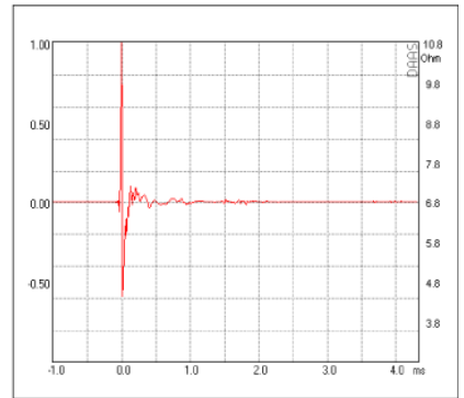
Impulse Response
