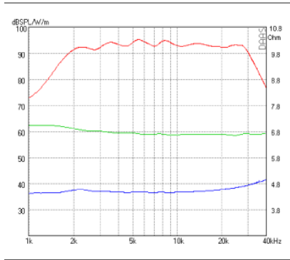
SPL 2.83 V - Phase - Impedance
