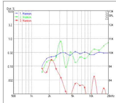
Harmonic Distortion 105 dB
